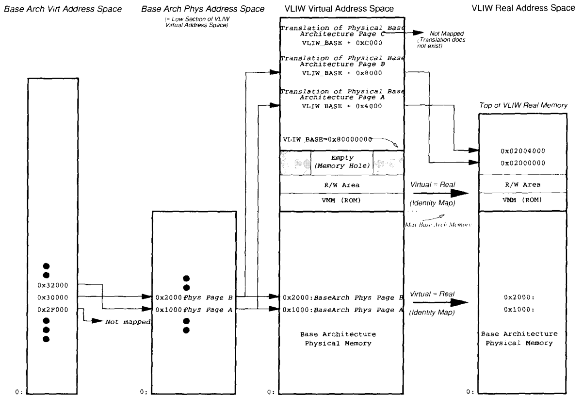
Figure 3.1: VLIW Address Space Layout
